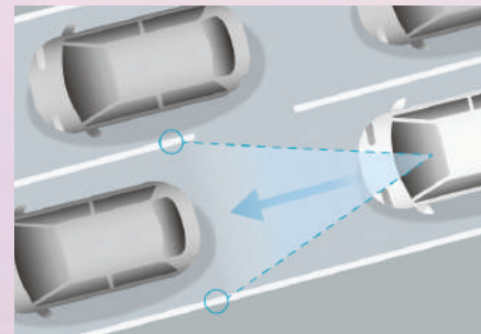
TRAFFIC JAM ASSIST
