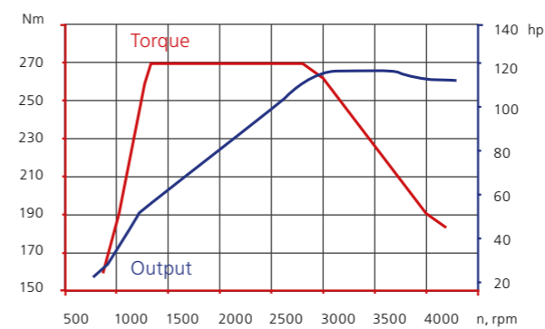
Diesel engine with 2.2 L displacement, 114 hp
