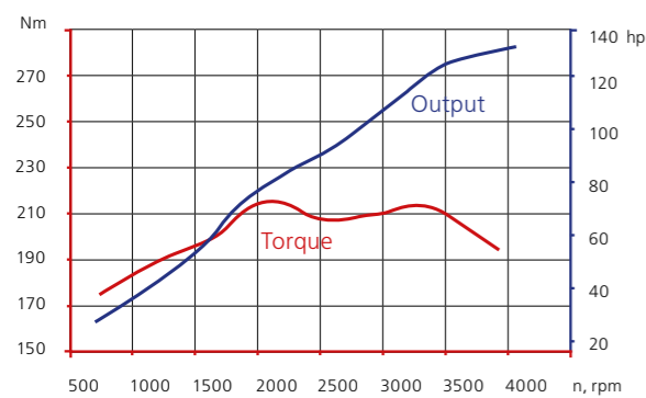
Petrol engine with 2.7 L displacement and 128 hp
