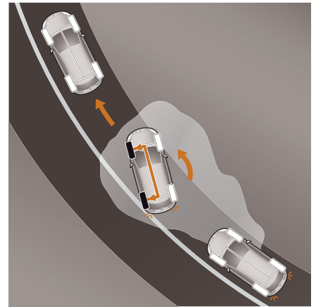
Electronic Stability Programme (ESP).
