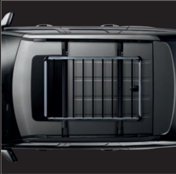
Luggage Carrier* LR006848 Load capacity 116lbs.
