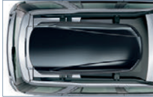
Luggage Box* VPLV/R0062 Gloss Black Finish. Opens from both sides. Lockable for security. External dimensions: 1,750mm long, 820mm wide, 450mm high. Volume 440 litres. Maximum payload 68kg**.
