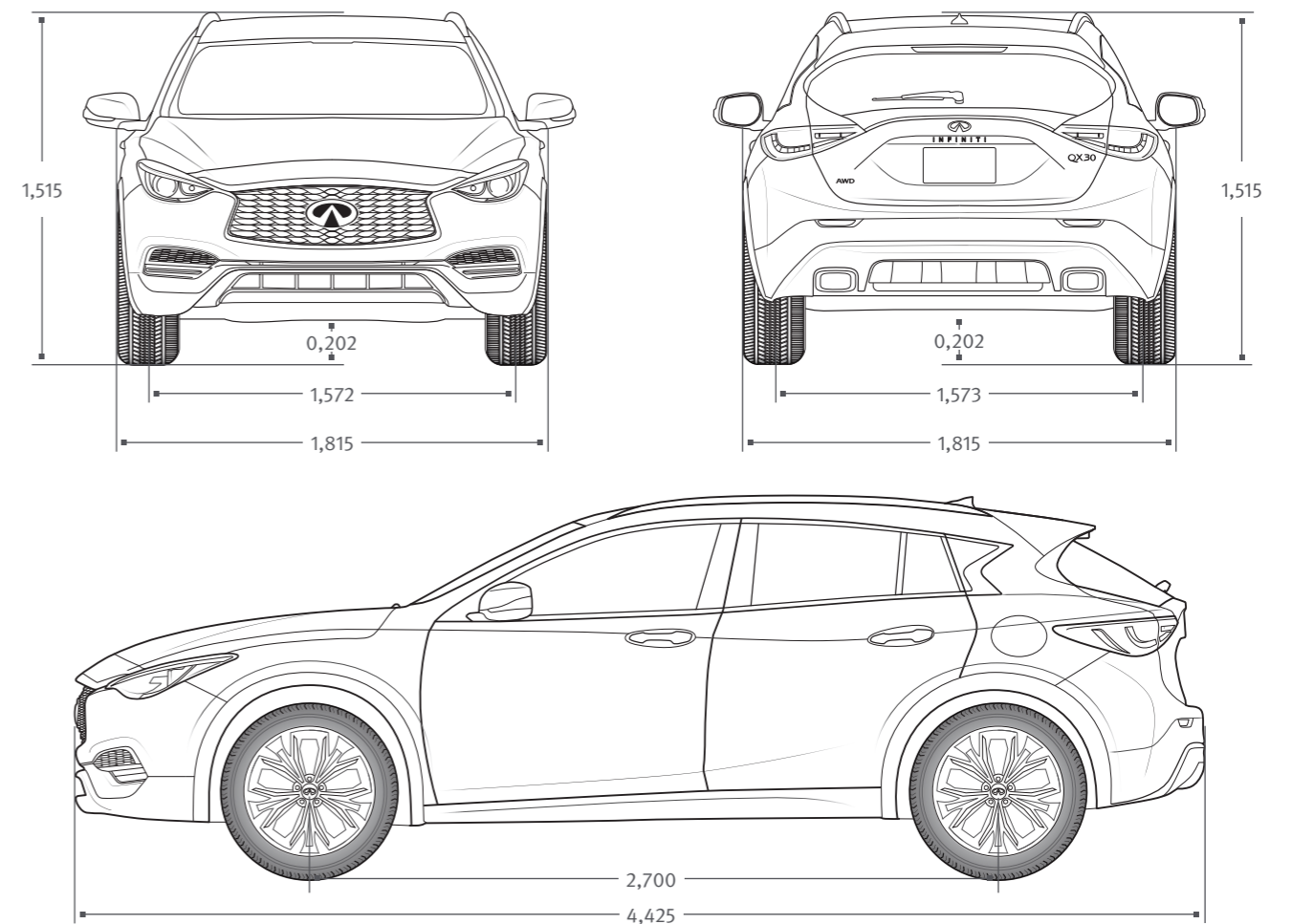
All dimensions are indicated in mm.
