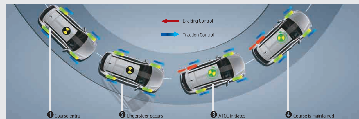
Advanced Traction Cornering Control (ATCC): While accelerating and turning frequently on highway interchanges and curves, ATCC distributes 4WD driving force and braking power. The VDC assesses torque vectoring information, and controls understeering, preventing the driver from overcompensating thereby improving agility and braking control.
