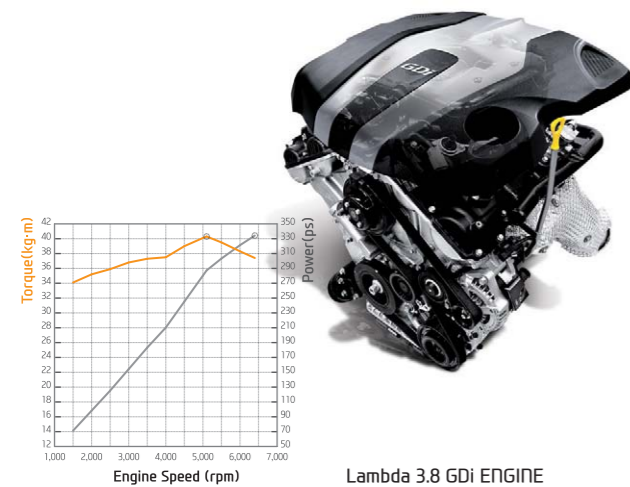
Lambda 3.8 GDI ENGINE
