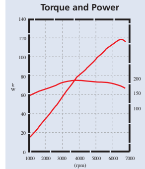
Flatter, more powerful torque curve for superior response
