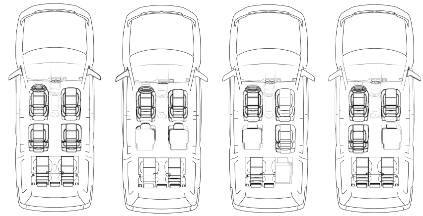
SEVEN-PASSENGER bucket seating. Two bucket seats in the second row and three-passenger 60/40 split-folding bench seating in the third row.
